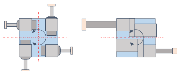
4 high-frequency spindles
